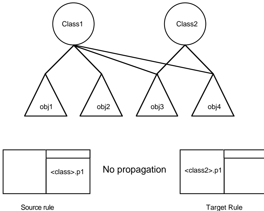
Figure 2-41 No Forward Action-Effects Between Dissimilar Class Patterns
