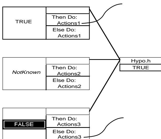
Figure 2-6 Multiple Rules Leading to One Hypothesis
