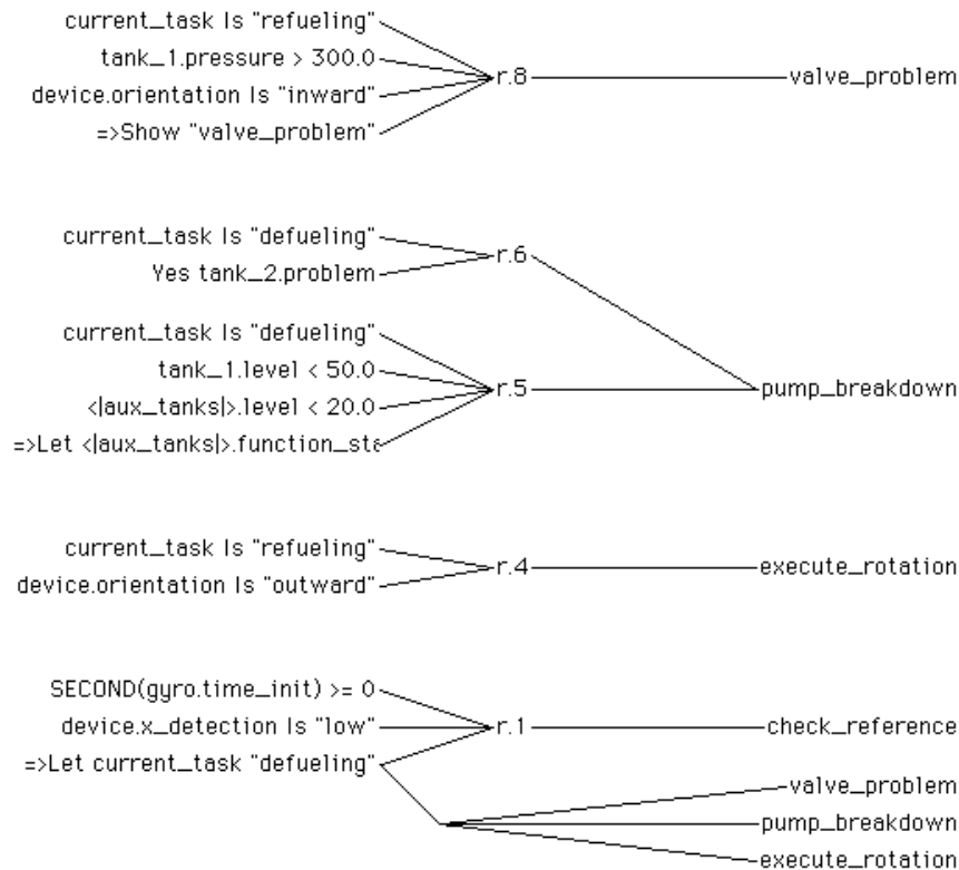
Figure A-14 Forwarding Data Can Cause Revisions
