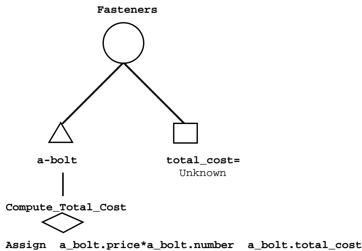
Figure 1-46 Inheriting an Explicit Method
