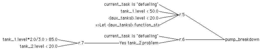
Figure A-3 Rules Linked by Subgoal Hypotheses
