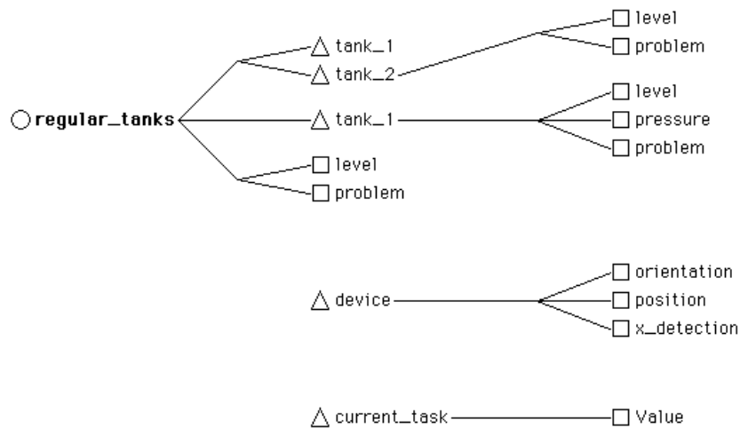
Figure A-11 Declared and Undeclared Object Structures
