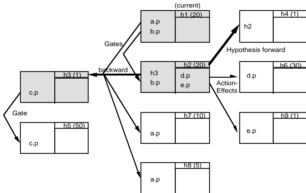
Figure 2-50 Action and Hypo Forward Generated Hypotheses
