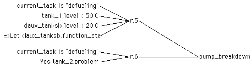
Figure A-2 Typical And/Or Rule Diagram
