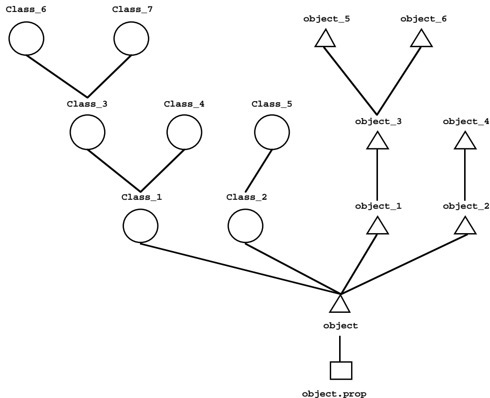
Figure 1-48 Conflict Resolution
