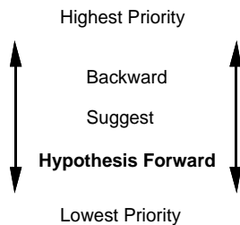
Figure 2-16 Agenda Priorities
