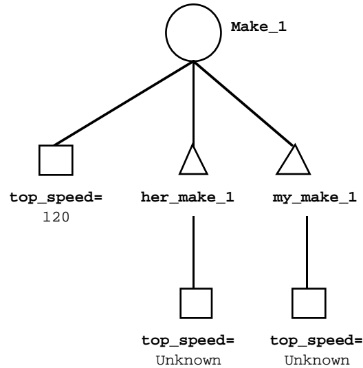
Figure 1-43 Value Inheritance
