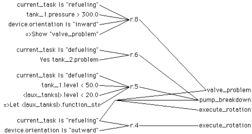
Figure A-7 Inductive Reasoning from Conditions (Forward Chaining)
