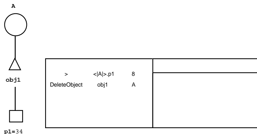
Figure 1-70 Deleting Objects Using Pattern Matching
