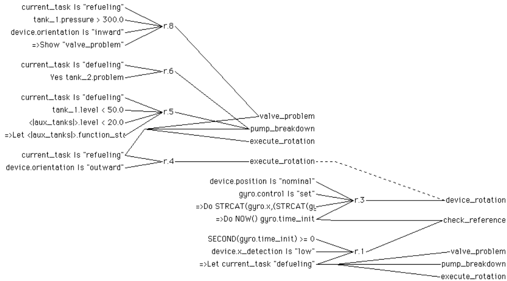
Figure A-10 Knowledge Islands Connected by Context Link
