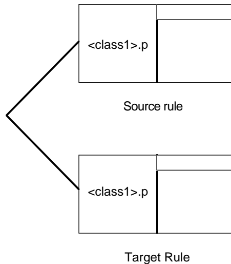
Figure 2-36 Gate Occurs on Same Patterns
