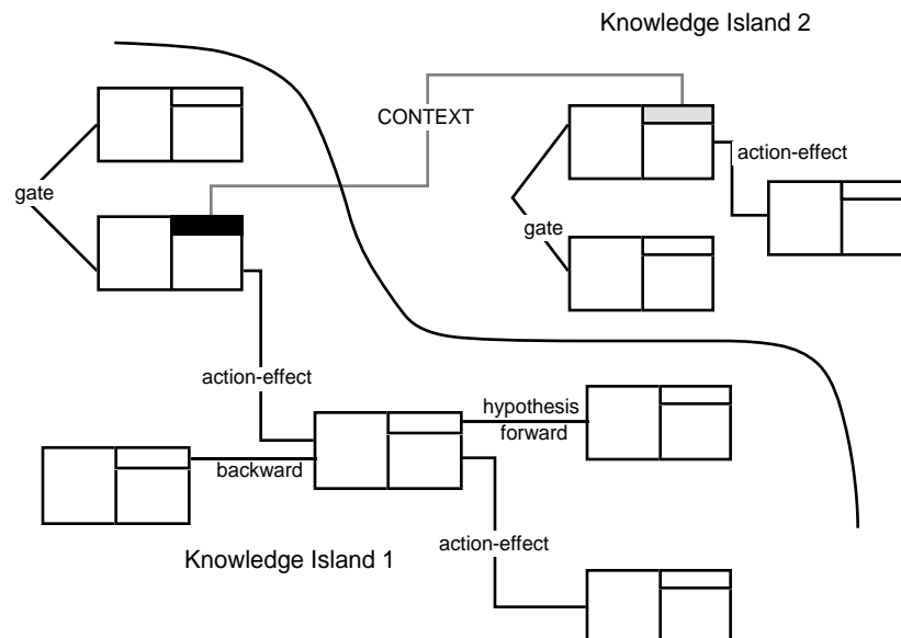
Figure 2-26 Knowledge Islands
