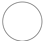
Figure 1-5 A Subclass
