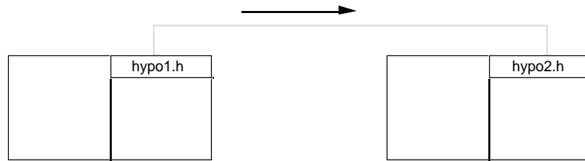
Figure 2-25 Context Link
