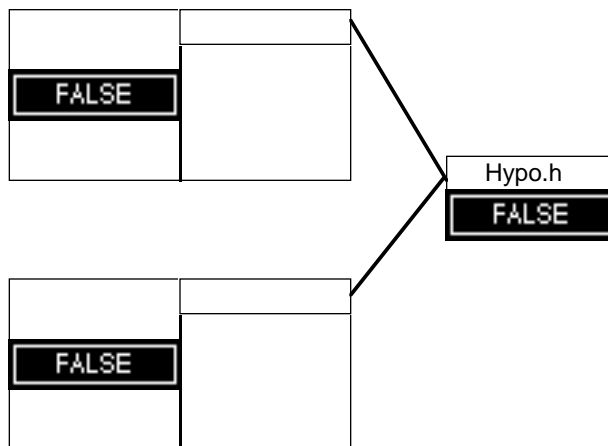
Figure 2-3 FALSE Rules
