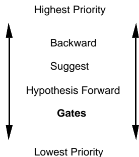
Figure 2-18 Agenda Priorities
