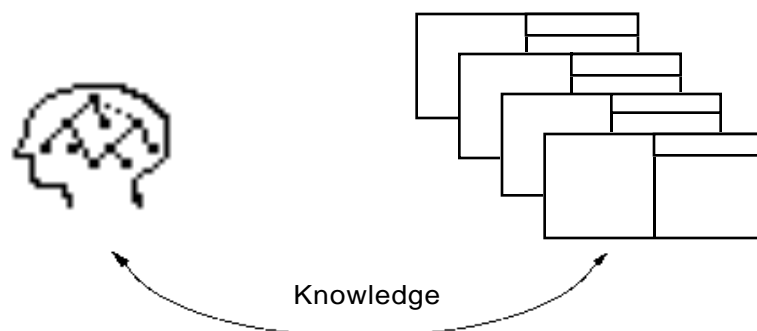
Figure 1-73 Transferring Knowledge
