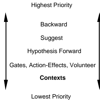
Figure 2–24 Agenda Priorities
