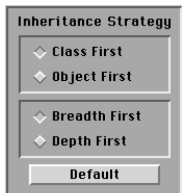
Figure 1-17 Inheritance Strategy
