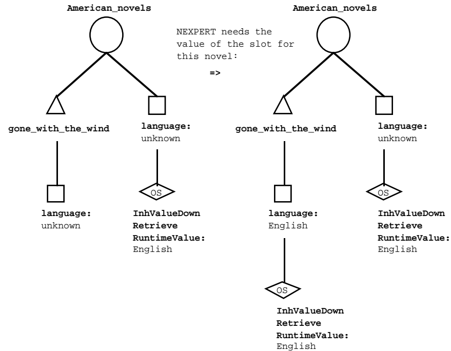
Figure 1-30 Method Inheritance
