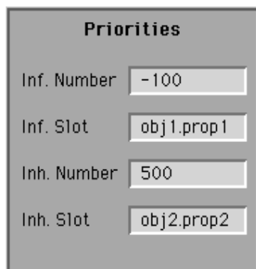
Figure 1-14 Inheritance Priorities
