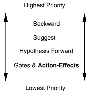
Figure 2-22 Agenda Priority
