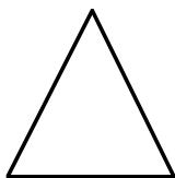
Figure 1-6 A Subobject
