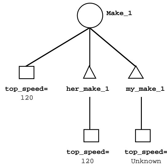
Figure 1-44 Value Inheritance
