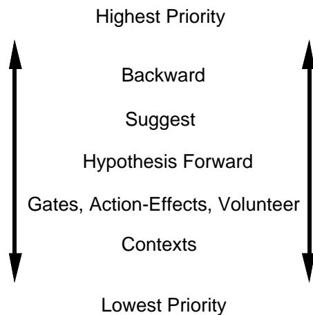
Figure 2-43 Agenda Priorities
