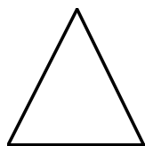
Figure 1-2 An Object
