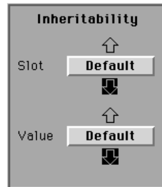
Figure 1-16 Class Inheritability
