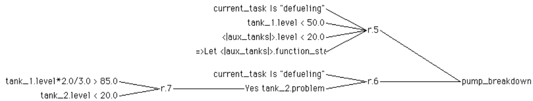
Figure A-4 Deductive Reasoning (Backward Chaining)
