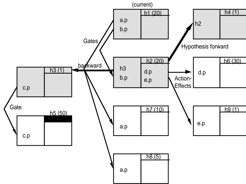
Figure 2-51 Refocusing on the Highest Priority Hypothesis
