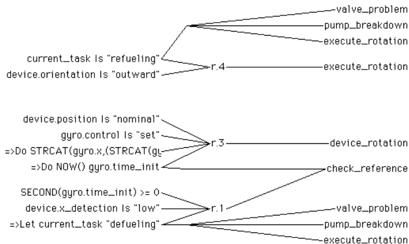
Figure A-8 Inductive Reasoning from Actions (Forward Chaining)
