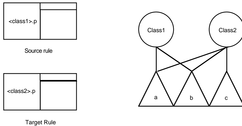
Figure 2-37 No Gate Occurs on Dissimilar Patterns
