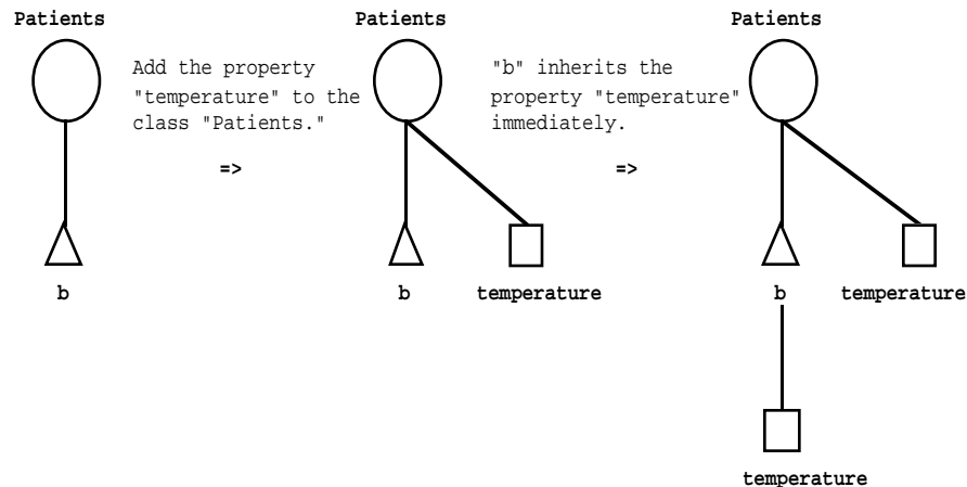
Figure 1-28 Property Inheritance
