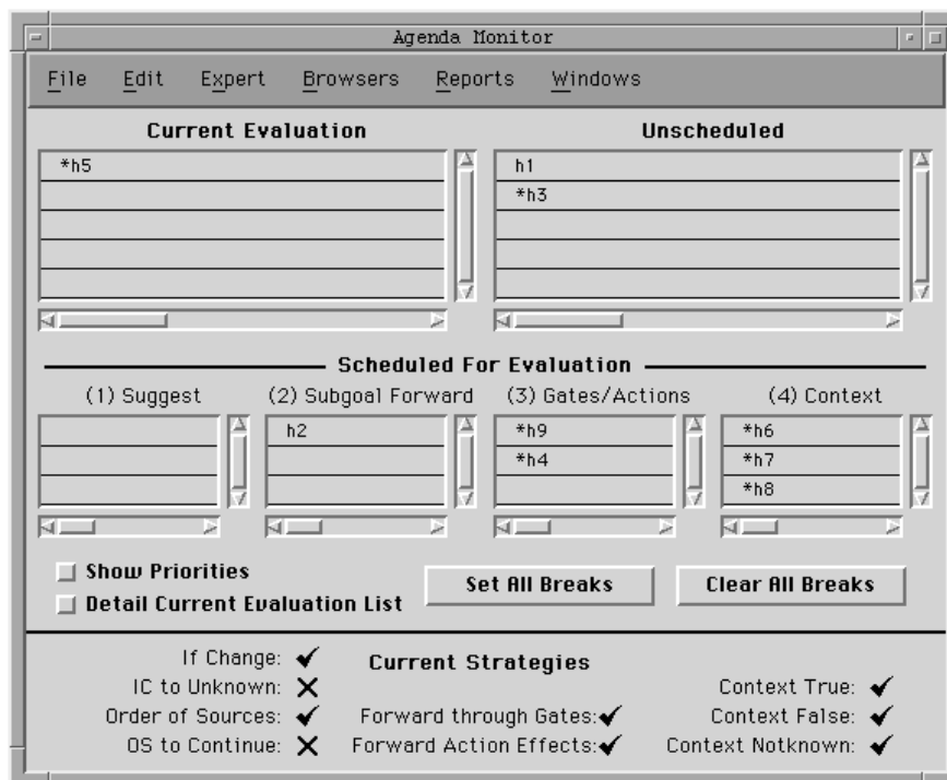
Figure 2-53 Agenda Monitor
