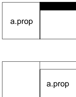
Figure 2-62 Revisions
