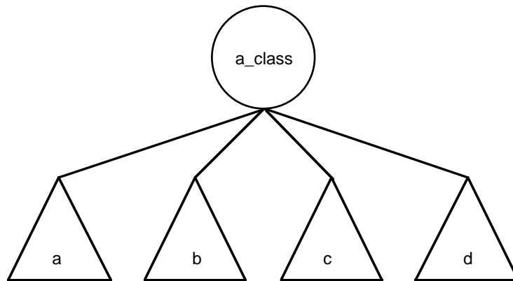
Figure 2-38 Class/Object Structure
