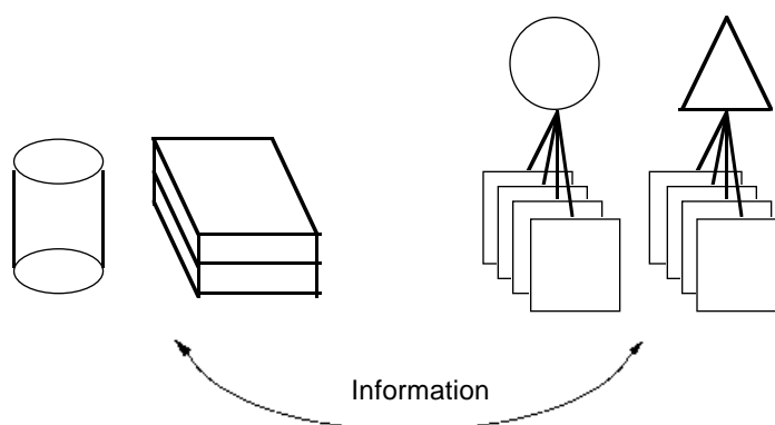
Figure 1-72 Transferring Information
