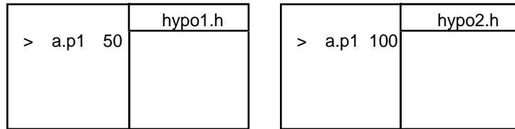
Figure 2-17 Gates
