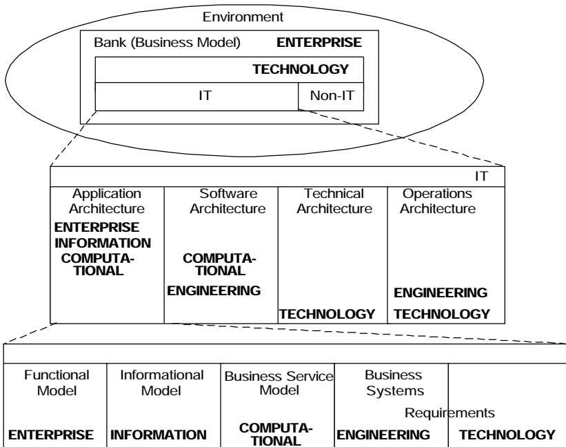
Figure 2. Nesting of Viewpoints
